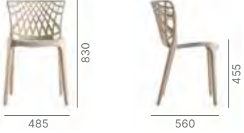
Tag 300 chair sedia Tag 300
